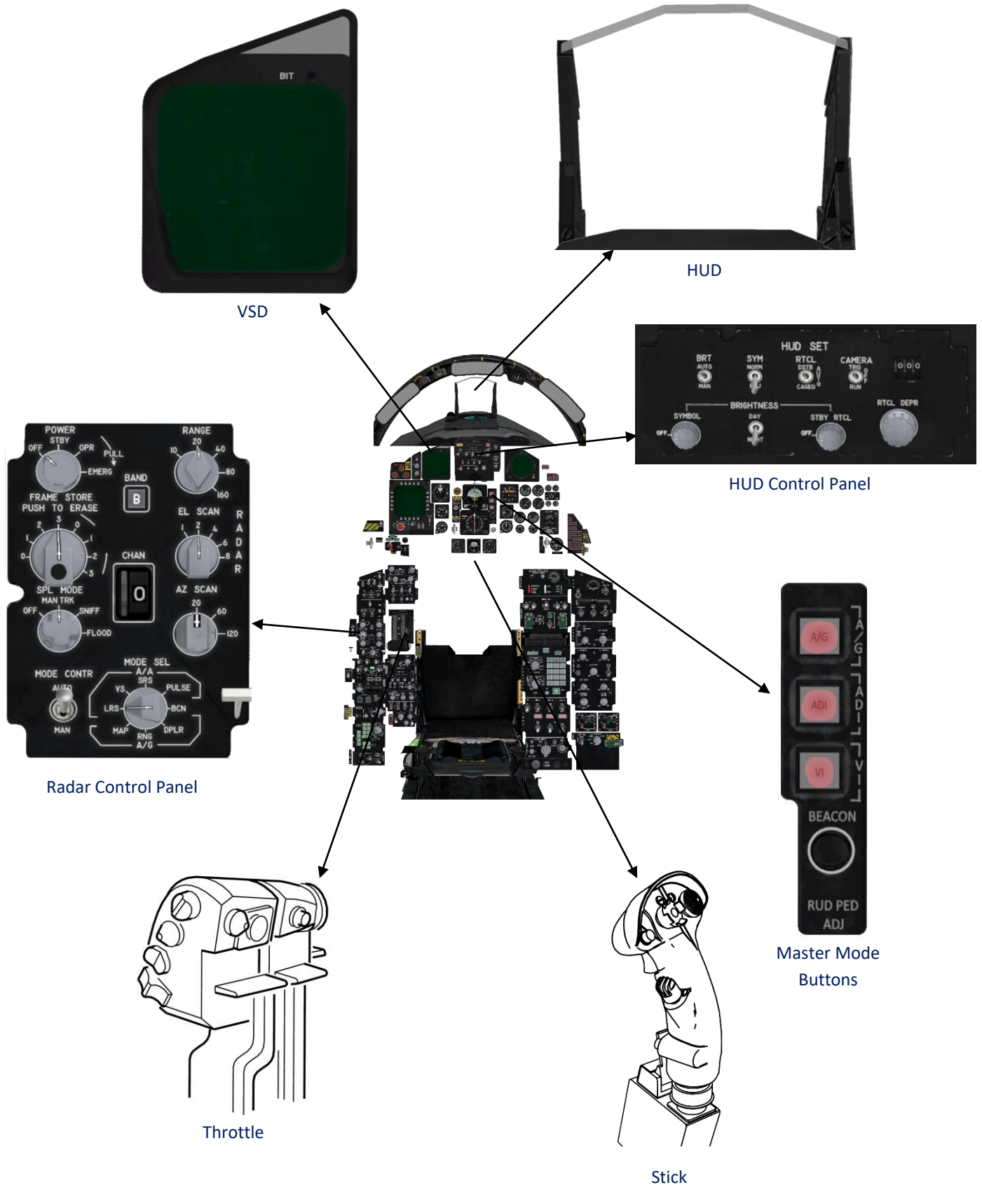
A/A FIRE CONTROL &amp; DISPLAY SYSTEMS
