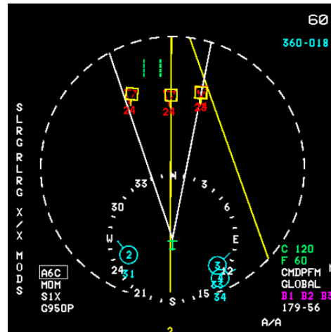
- RADAR IN TRACK WHILE SCAN - ALL PREVIOUS SURV TRACKS NOW SUPERIMPOSED WITH FIGHTER TRACK SYMBOLS
