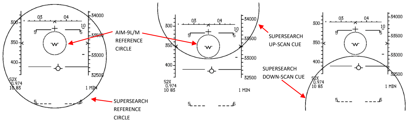
1. SUPERSEARCH, SRM SELECTED
