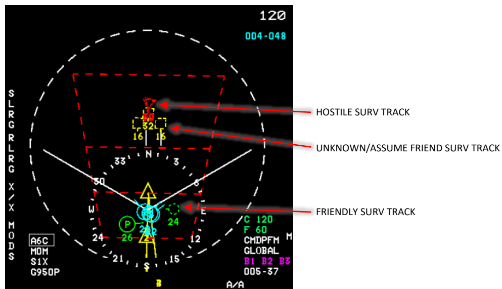
TYPICAL SIT DISPLAY WITH SURV TRACK PRESENTATION.
