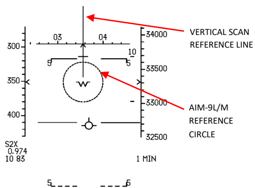
6. VERTICAL SCAN, SRM SELECTED
