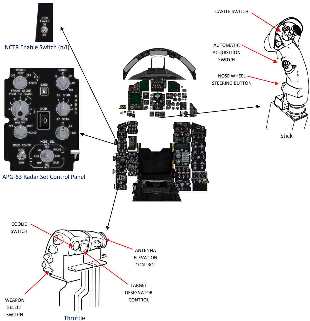
Radar Controls
